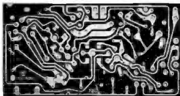
Printed circuit of copper on baseboard, before components are assembled.
